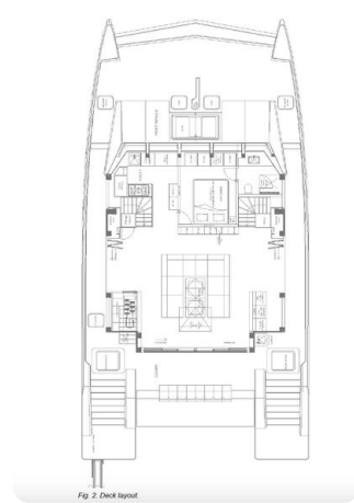
Fig. 2. Deck layout.
