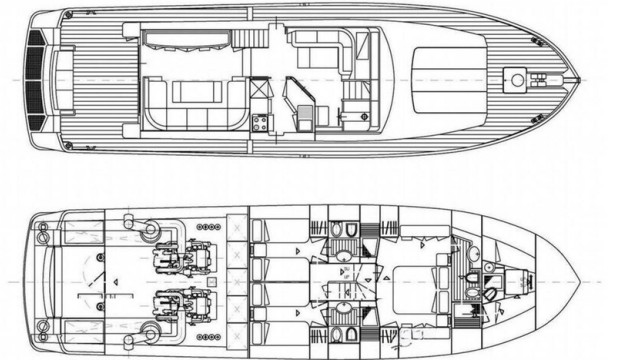
SANLORENZO SL 62 layout
