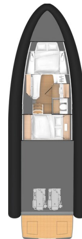
Strider15-Lower-Deck
