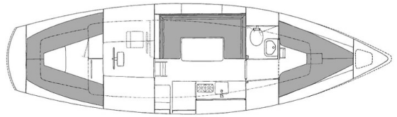
layout HR 35 Rasmus
