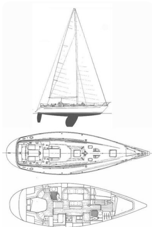
Grand Soleil 45 Layout
