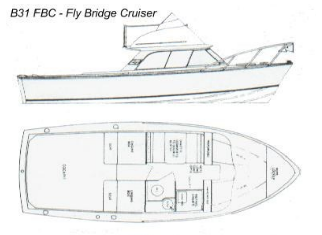
Bertram 31 Fbc layout
