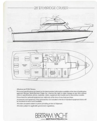
Bertram 28 Fbc plan
