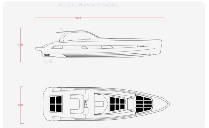
DOCKING PLAN
