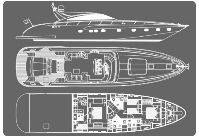
AB Follia 75 s layout
